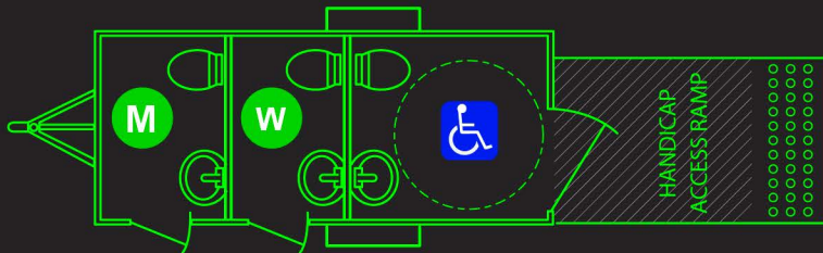
Trailer Dimensions: 14' L x 6' W x 11'6" H
